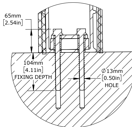
Fixing Detail
